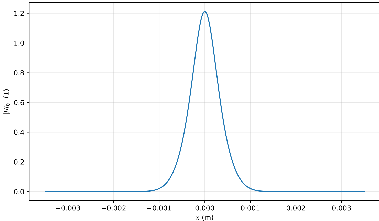
Intensity profile I(x, y = 0, z = 0.557m)/I_0 , P_{in}=1.0P_{cr} , artificial time
